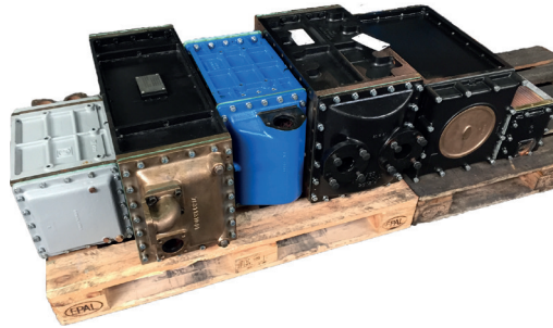
Overhauled and u ultrasonically cleaned air coolers.
